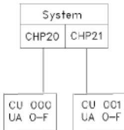
Figure 39. ESCON control units requiring unit address 00
