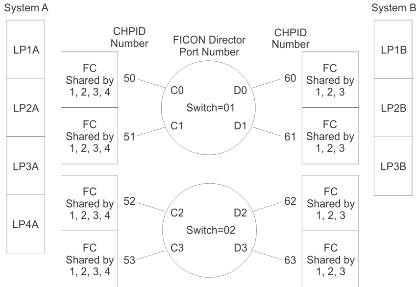
Figure 46. FICON CTC (fully redundant)
