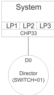
Figure 33. FICON CTC and director with single path
