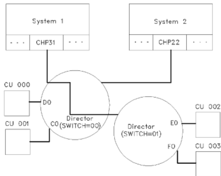
Figure 34. Chained ESCON directors
