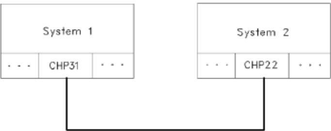
Figure 31. ESCON CTC point-to-point
