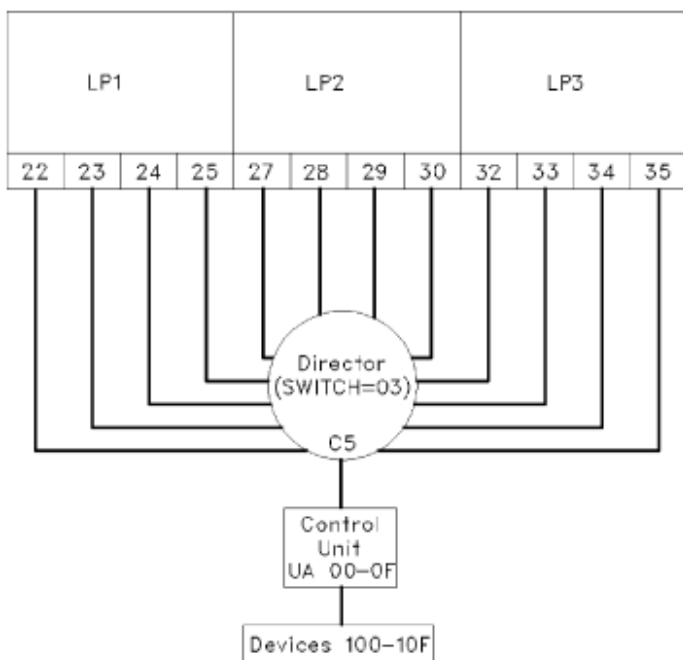
Figure 29. LPAR mode with more than eight paths to an ESCON device
