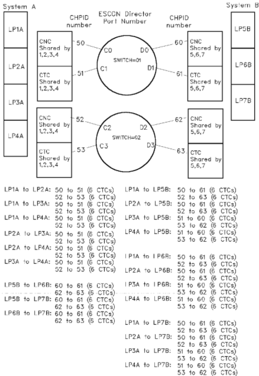
Figure 45. ESCON CTC with shared channels
