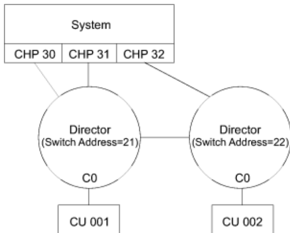
Figure 35. Cascaded FICON directors
