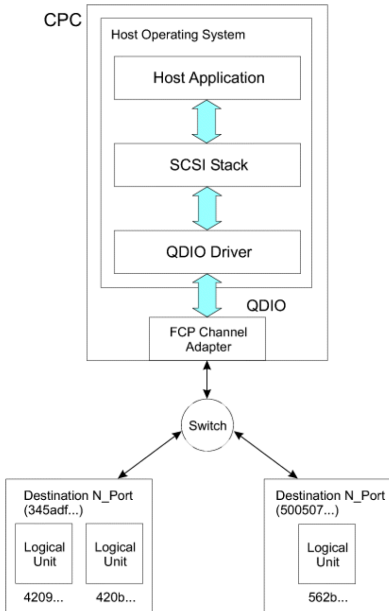
Figure 42. FCP channel configuration
