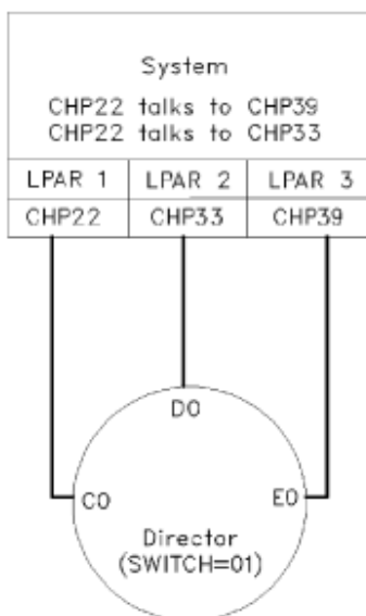
Figure 32. ESCON CTC dynamic through an ESCON director with multiple paths
