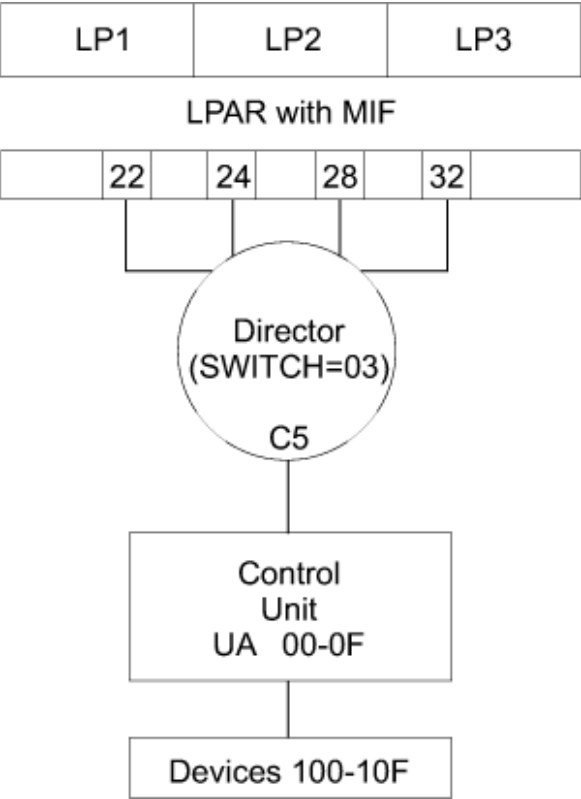
Figure 30. LPAR mode with shared paths to an ESCON device
