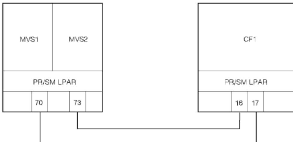
Figure 43. Coupling facility configuration
