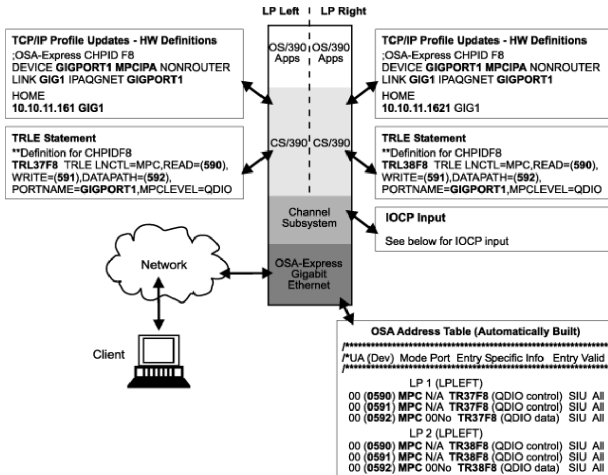
Figure 40. OSA configuration with two logical partitions
