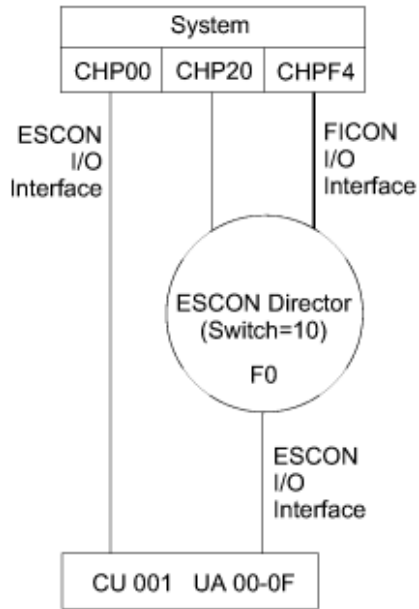
Figure 38. FCV channel configuration
