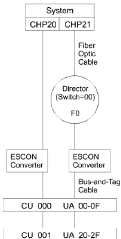
Figure 37. Channels through an ESCON converter
