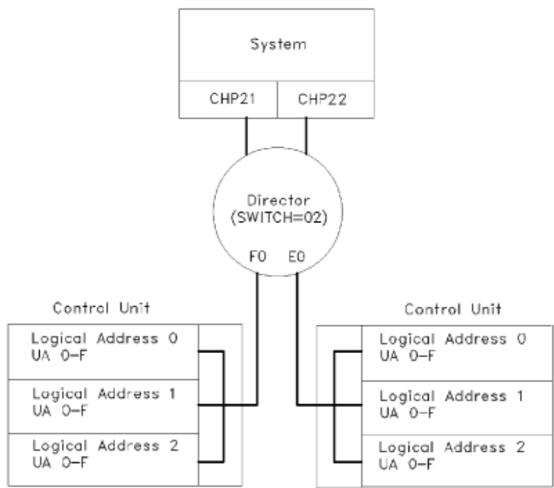
Figure 36. Control unit logical addressing
