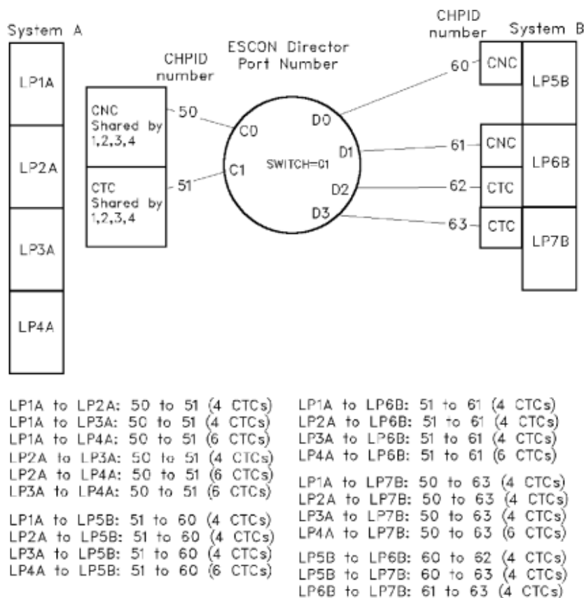
Figure 44. ESCON CTC with shared and unshared channels
